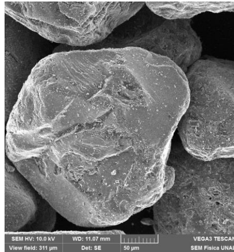
Figure 2. Micrographs SEM of black sand (M2 fraction) used as semiconductor during MO photocatalytic oxidation.
